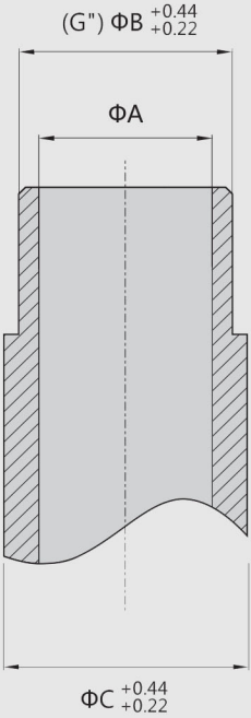
In Line Solenoid Pulse Valve pipe diameter
