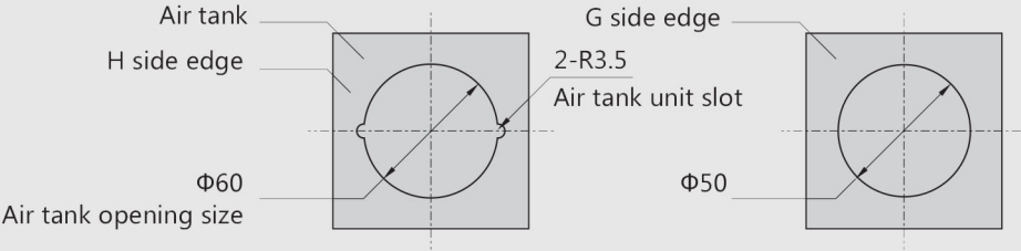
RMF-Y-25 Valve and air tank installation dimension
