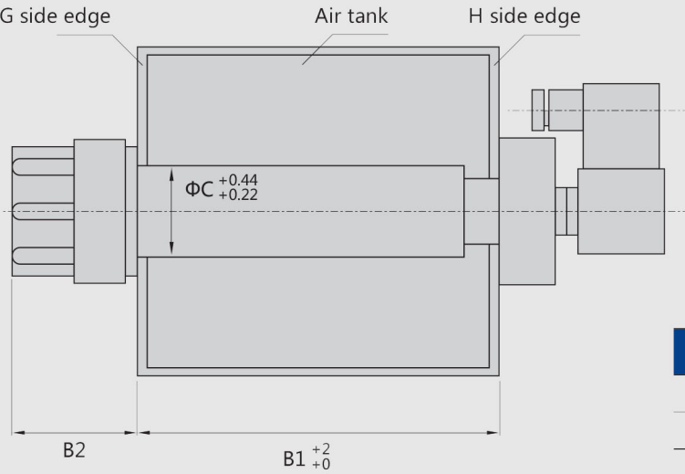
RMF-Y-25、RMF-Y-40 Installation method
