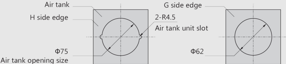
RMF-Y-40 Valve and air tank installation dimension
